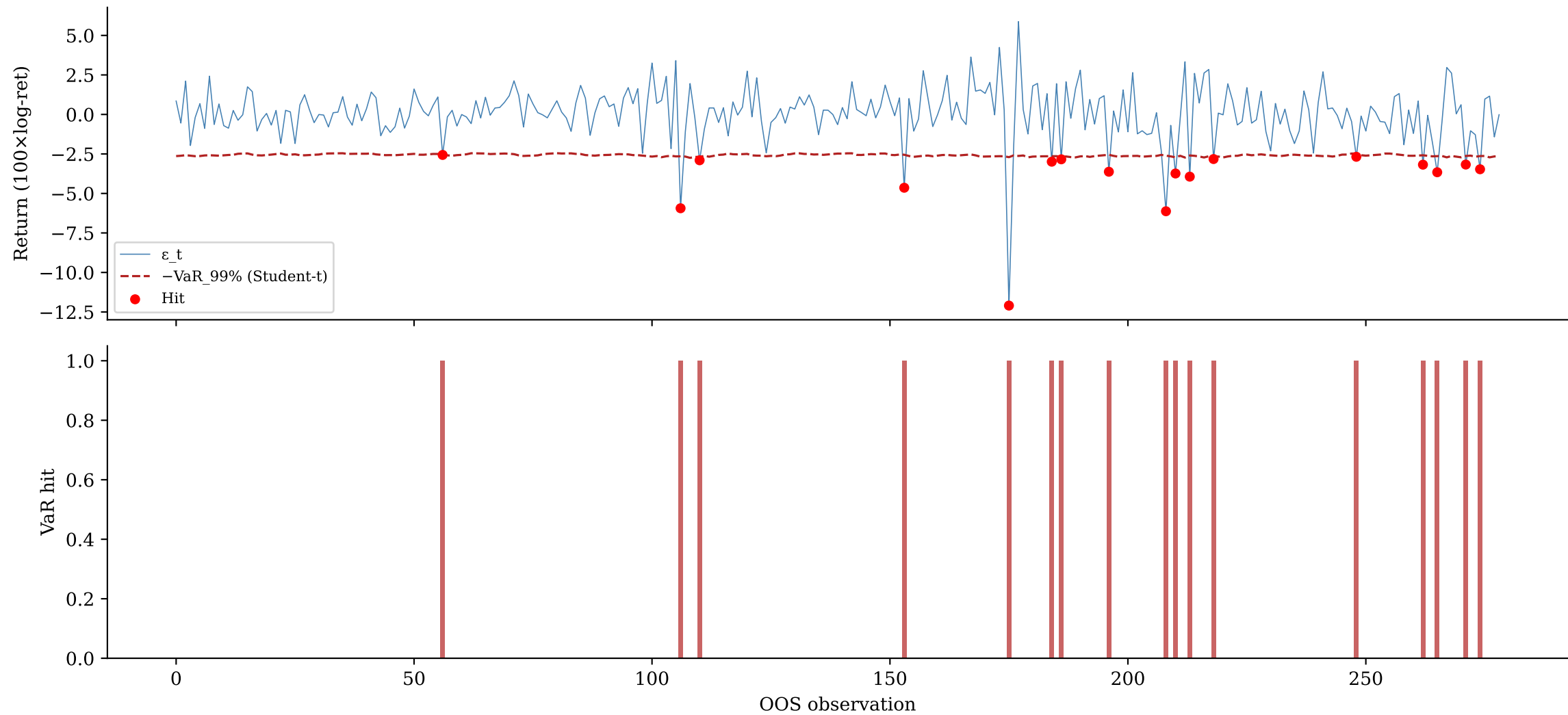
LSTM-SSE-t-Student — GOLD VaR 99% Hit Sequence
